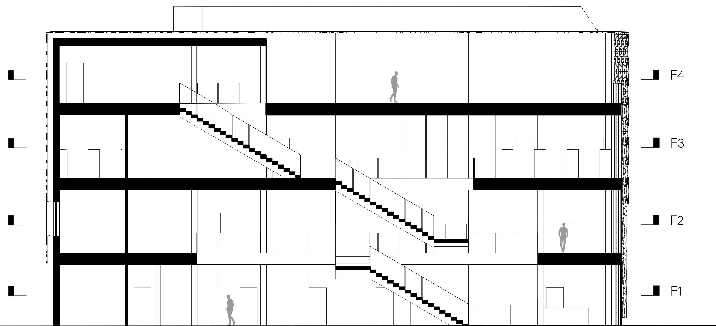
SECTION 2 1' = 1/8"
