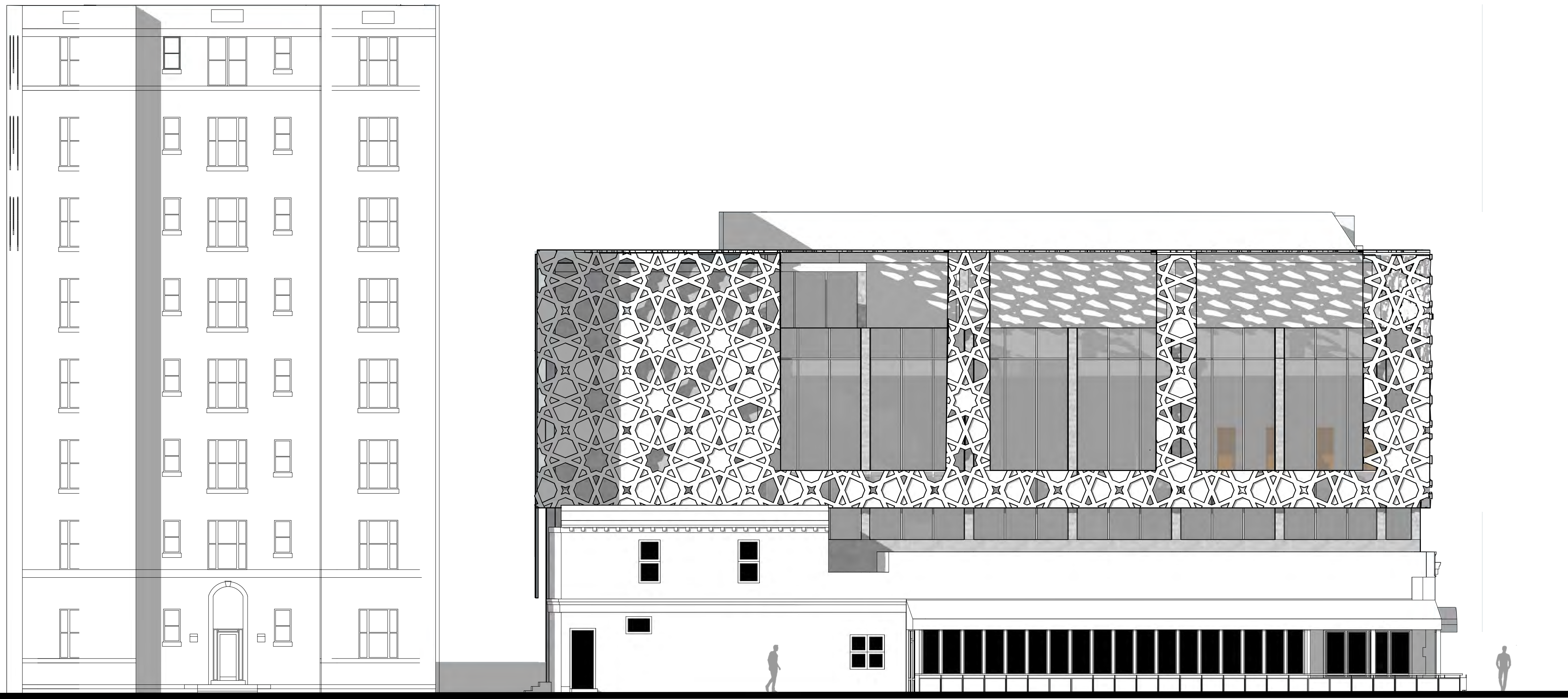
NORTH ELEVATION 1' = 1/8"
