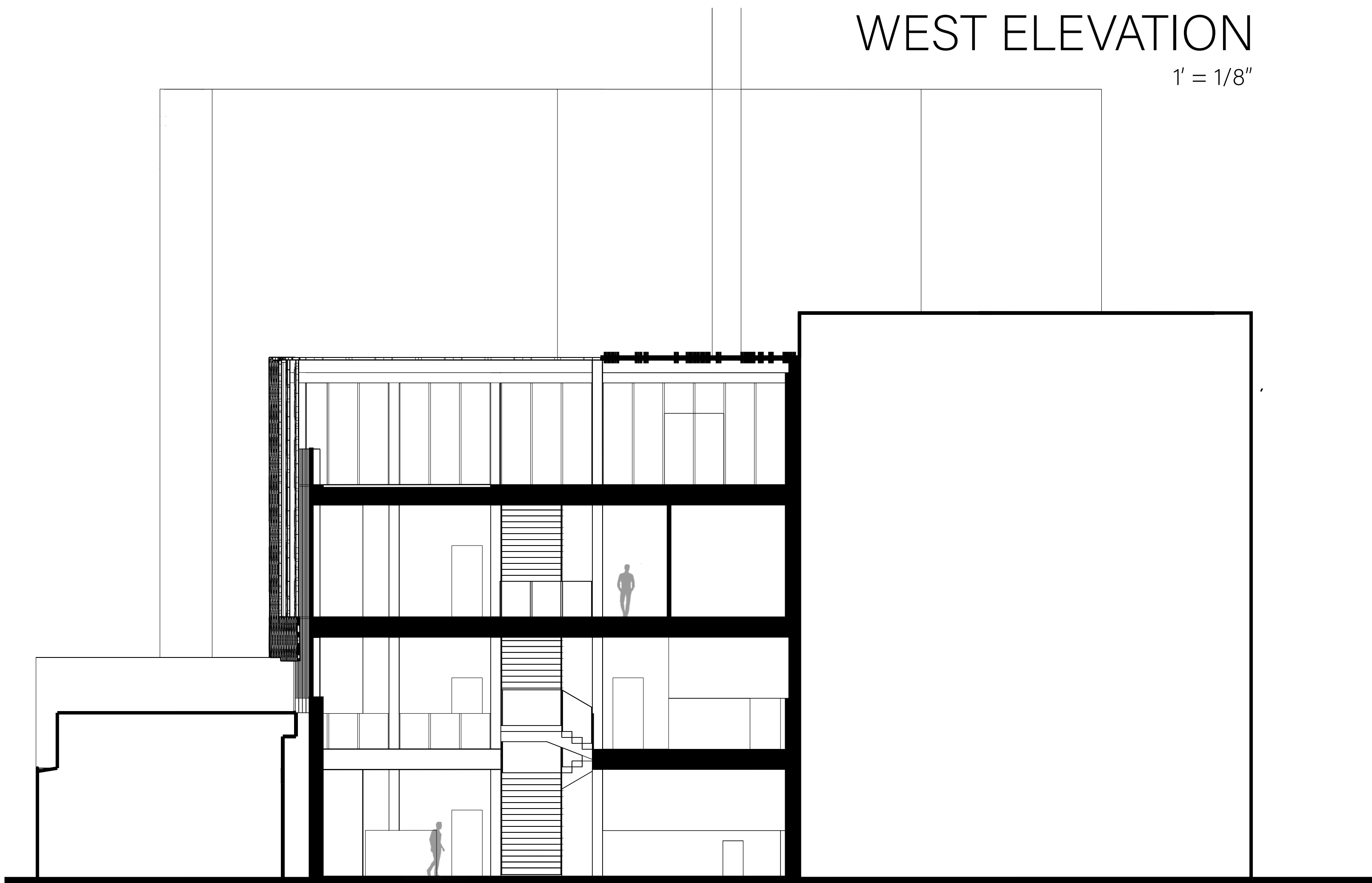
SECTION 1
