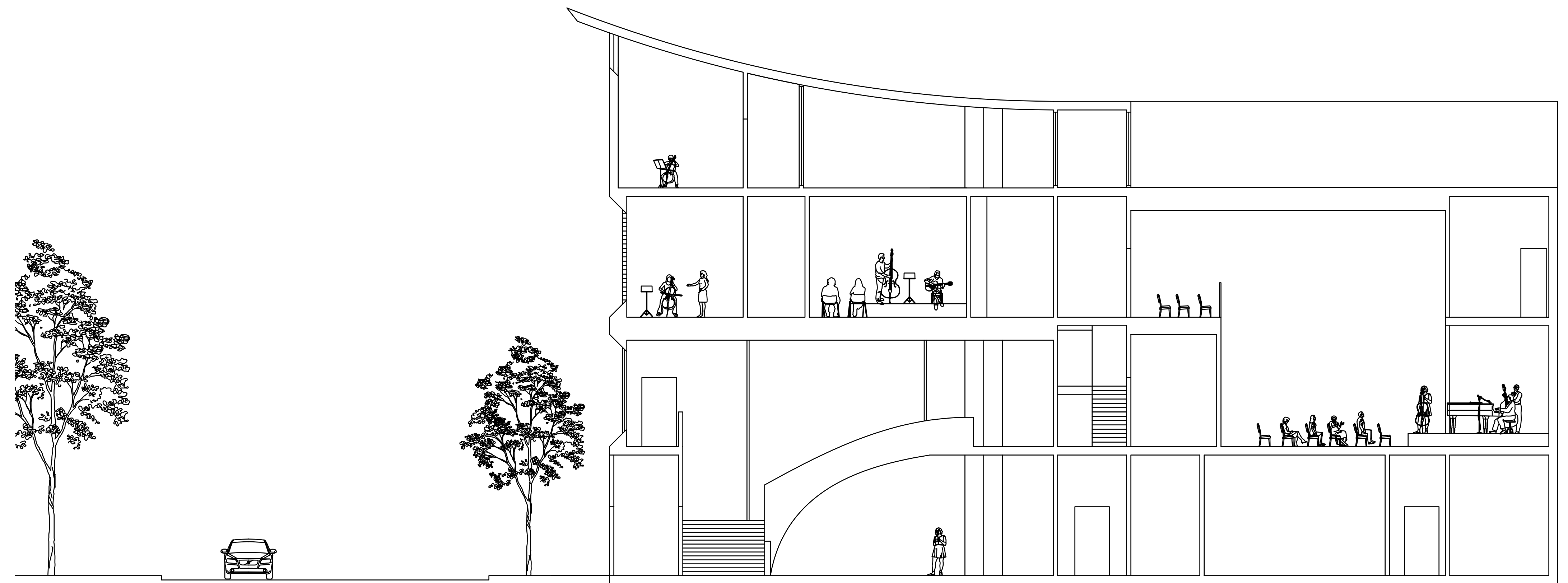
LONGITUDINAL SECTION LOOKING WEST
