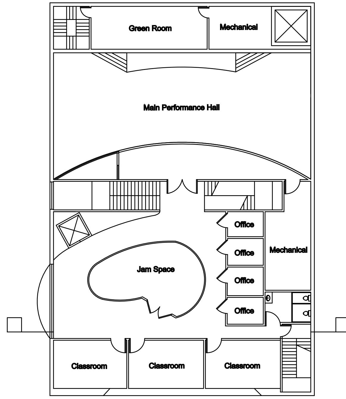
LEVEL THREE
