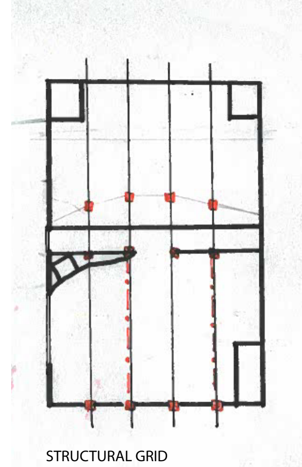
STRUCTURAL GRID
